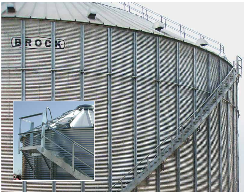
SHUR-STEP® Stairs can be used with stiffened or unstiffened bins, or bins with wind rings.
