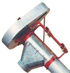
BROCK® Universal Parts Kit allows the incline angle of the Rigid Auger System to be adjusted.
